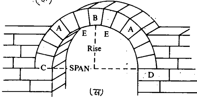
Arch and its parts
