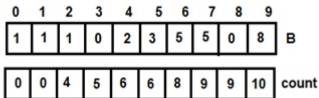
Figure 3.11: For i=7
