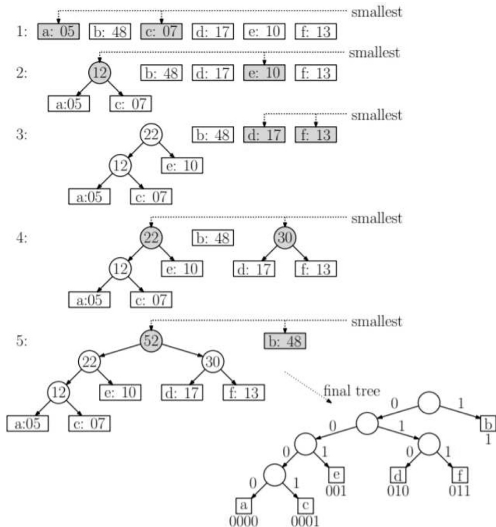
Fig. 4.2 Huffman Coding
