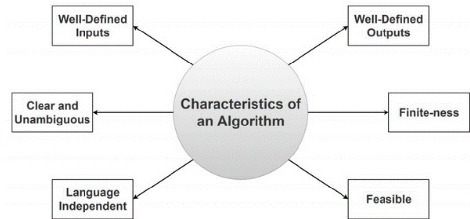
Figure 1.2: Algorithm Characteristics
