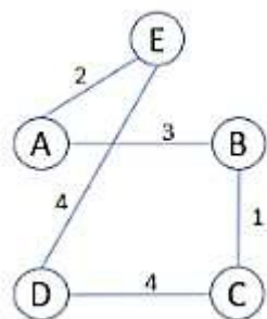
Figure 6.4: Weighted Graph
