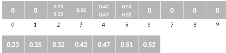
Figure 3.25: Gather elements from each bucket
