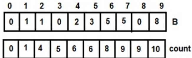
Figure 3.10: For i=6
