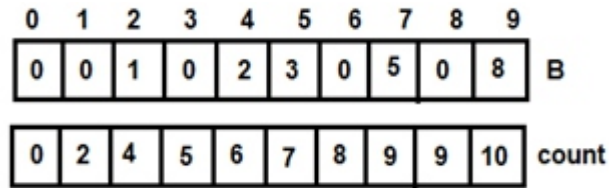
Figure 3.8: For i=4
