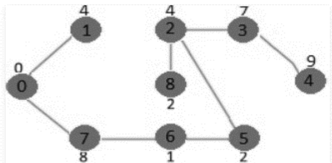
Fig. 4.8 Prim's Algorithm
