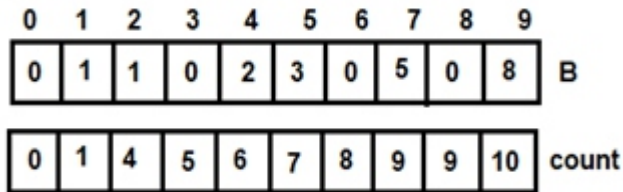
Figure 3.9: For i=5
