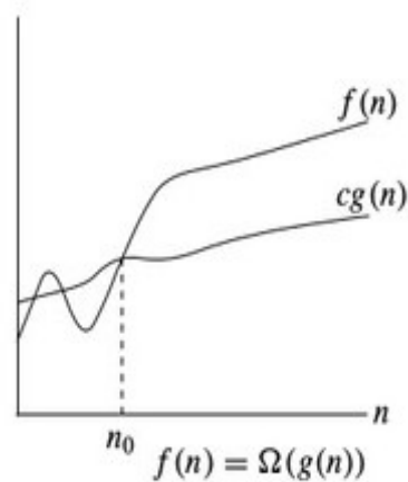
Figure 1.4: \Omega Notation
