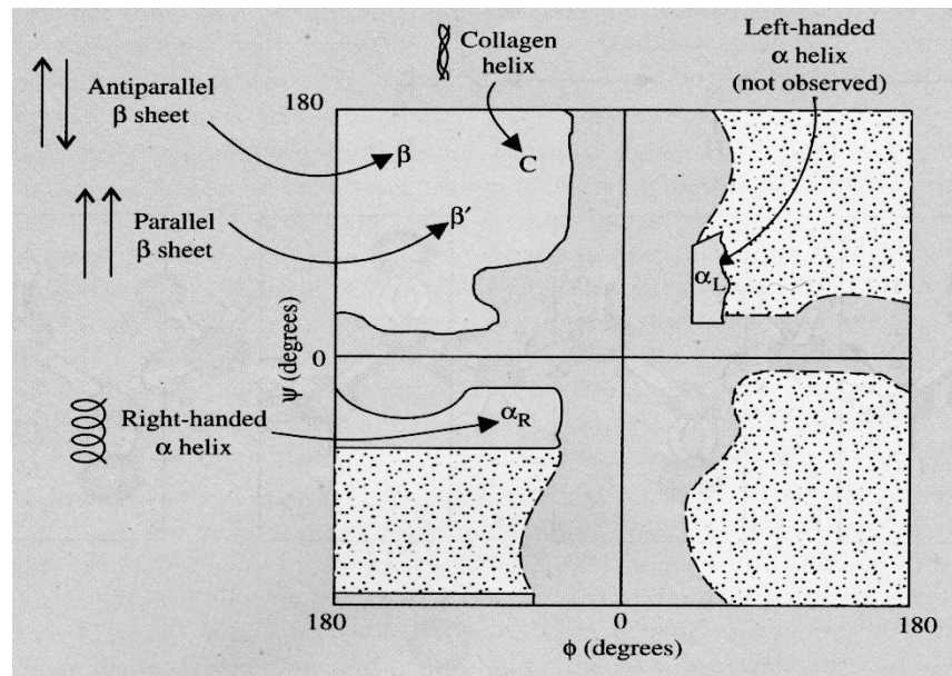
Fig.5.2: Ramachandran Plot
